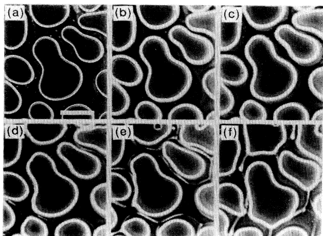
FIG. 4. Pattern evolution caused by a double quench ( 22.0^{\circ}\text{C} , 3600 s, 6.8^{\circ}\text{C} ) ( 162.0^{\circ}\text{C} , 168.0^{\circ}\text{C} ) in a PS-PVME (50-50) mixture. (a) -10 s, (b) 300 s, (c) 900 s, (d) 1500 s, (e) 3600 s, and (f) 9000 s after the second quench. The bar corresponds to 10\ \mu\text{m} .
